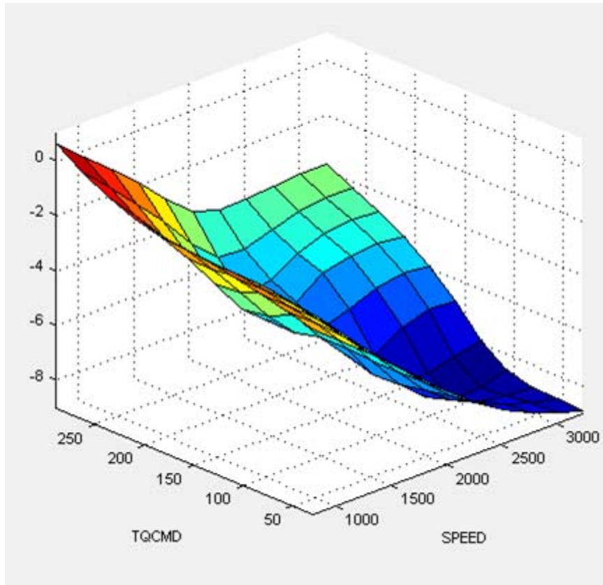
Main Start of Injection (SOI) Timing Table
