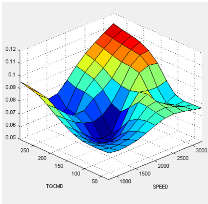
Pilot Fuel Mass Fraction Table
