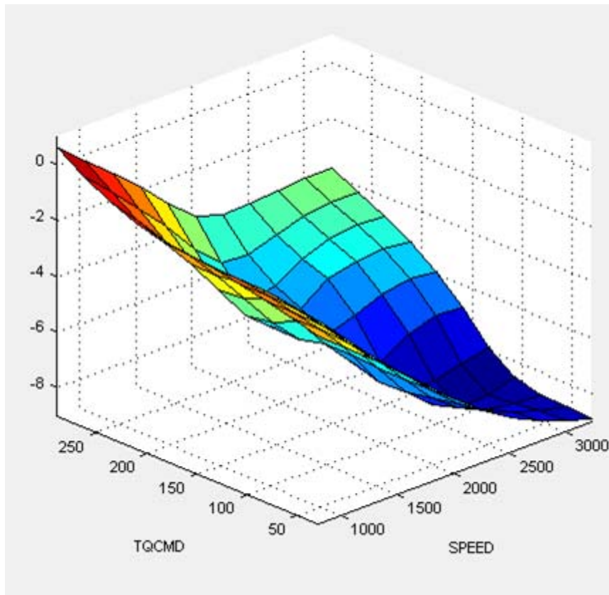
Main Injection Timing (SOI) Table
